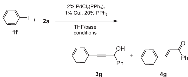
Scheme 5. CIR of iodobenzene ( 1f ) and 2a under dielectric and conductive heating.
