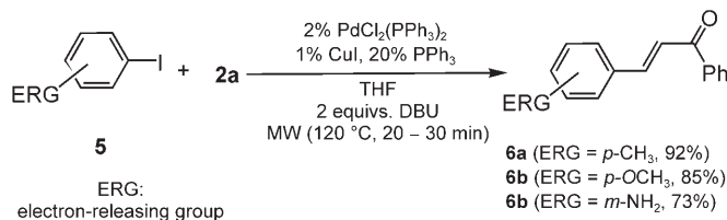
Scheme 6. MACIR of electron-rich iodobenzenes 5 and 2a .
