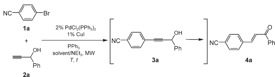
Scheme 2. MACIR of p -bromobenzonitrile ( 1a ) and 1-phenylpropyn-1-ol ( 2a ).
