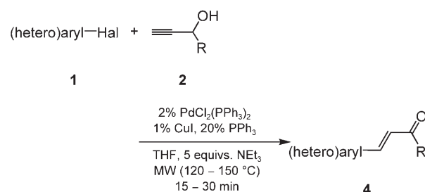
Scheme 4. MACIR of (hetero)aryl halides 1 and propargyl alcohols 2 .
